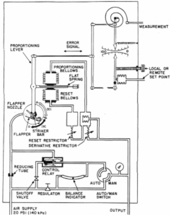
Controller with Proportional, Reset, and Derivative Actions, and Automatic-Manual Transfer System (Optional)
