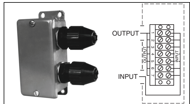
Figure 6. Junction Box
