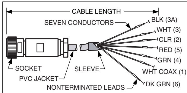
Figure 7. Patch Cord
