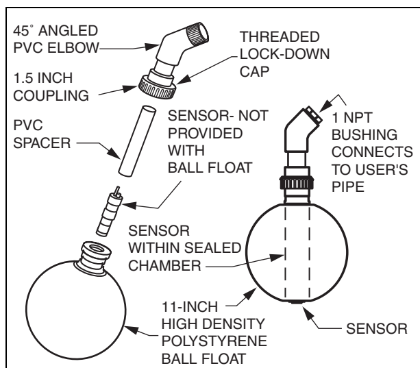
Figure 9. Ball Float Assembly Membrane Replacement Kits for 871DO-C Probes
