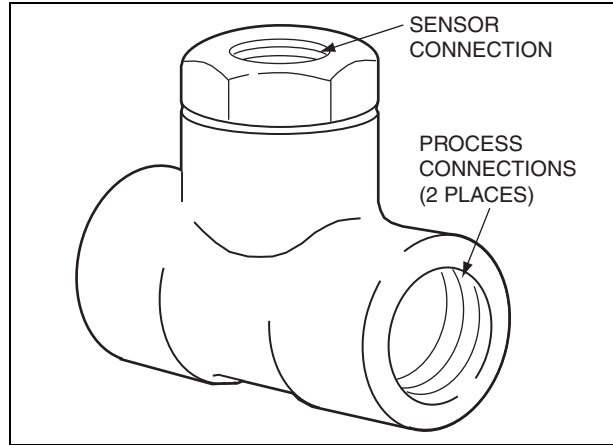
Figure 4. Tee Assemblies
