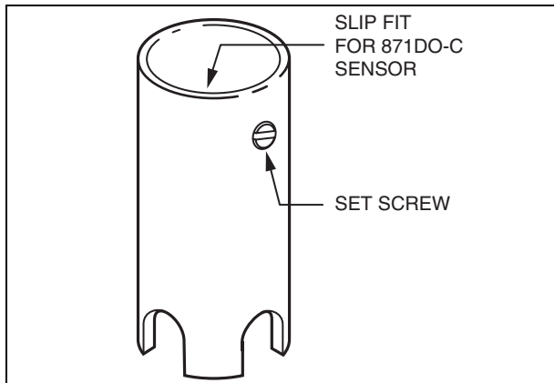
Figure 5. Electrode Protection Sleeve
