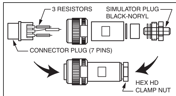
Figure 8. Cell Simulator
