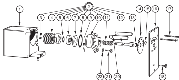
DERIVATIVE RESTRICTOR ASSEMBLY (FIGURE 10)
