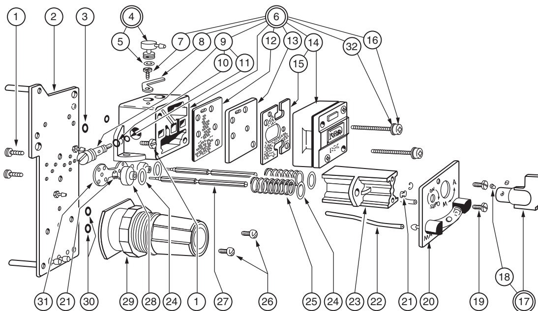
AUTO-MANUAL TRANSFER SYSTEM (FIGURE 5 - Also see Item 21, Figure 1)
